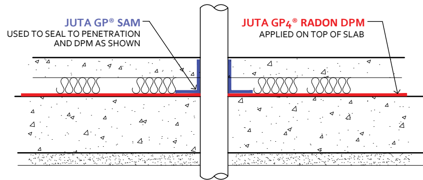
PIPE PENETRATION WITH SELF ADHESIVE GAS MEMBRANE
