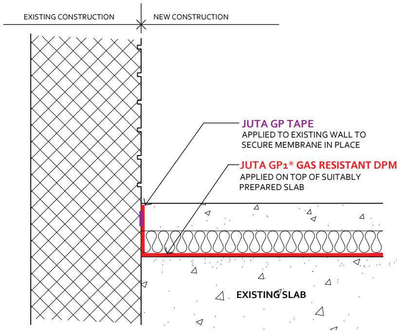
OPTION 2: SEAL TO EXISTING MASONRY USING DOUBLE SIDED TAPE
