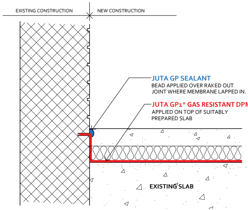
OPTION 1 (PREFERRED SOLUTION): RAKE OUT MORTAR JOINT & SEAL USING JUTA GP SEALANT
