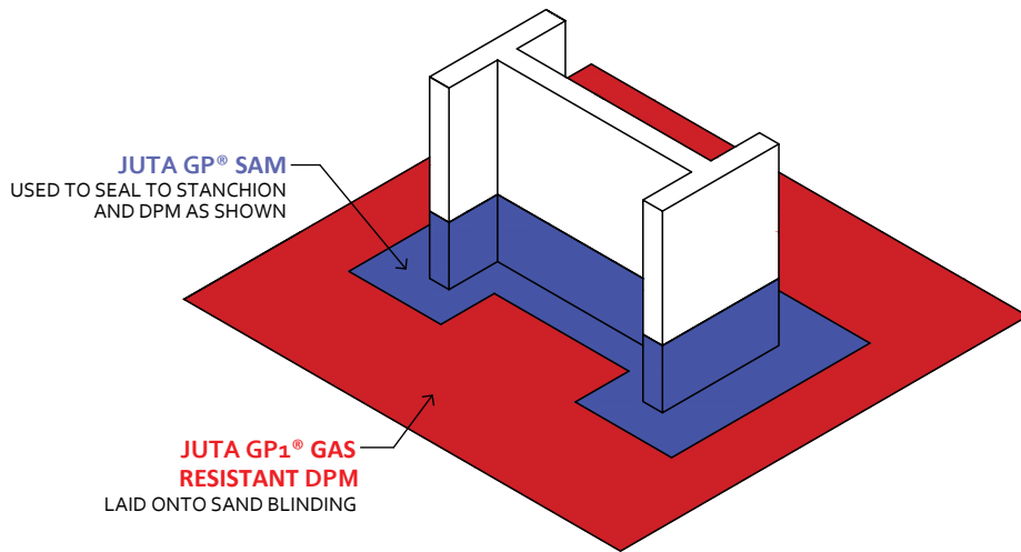
NB - PLEASE REFER TO TD-JUTA.GP1.042 FOR STANCHION SEALING OPTIONS FOR GP1.
