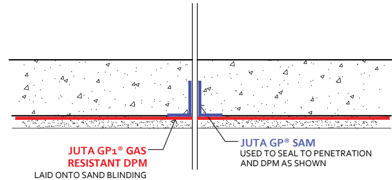
ROD/ REBAR/ HANGAR WITH SELF ADHESIVE GAS MEMBRANE
