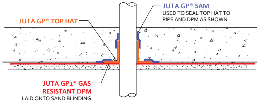
PIPE PENETRATION WITH TOP HAT DETAIL
