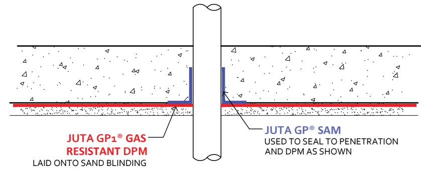
PIPE PENETRATION WITH SELF ADHESIVE GAS MEMBRANE
