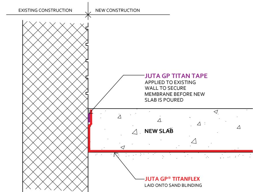
OPTION 2: SEAL TO EXISTING MASONRY USING DOUBLE SIDED TAPE
