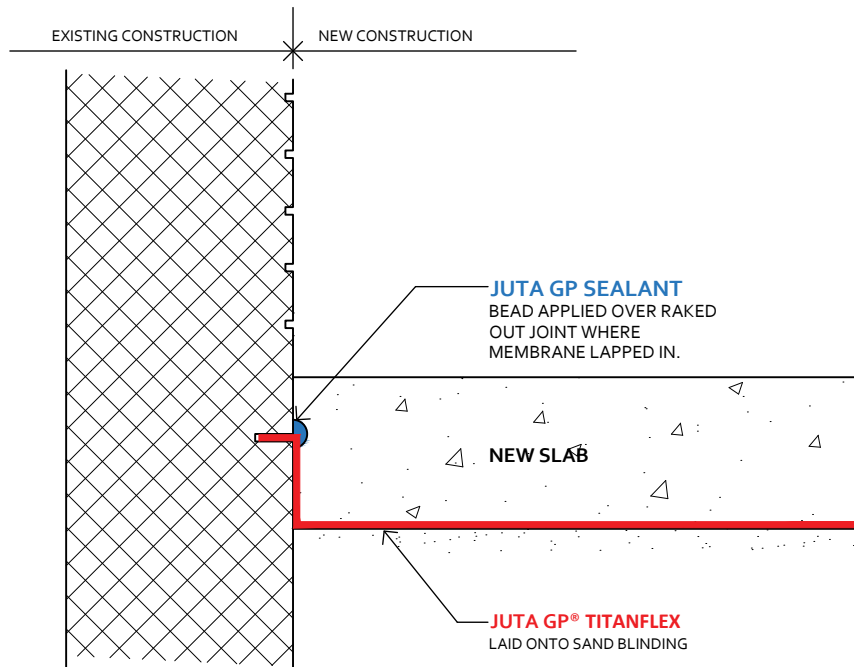
(PREFERRED SOLUTION) OPTION 1: RAKED OUT MORTAR JOINT
