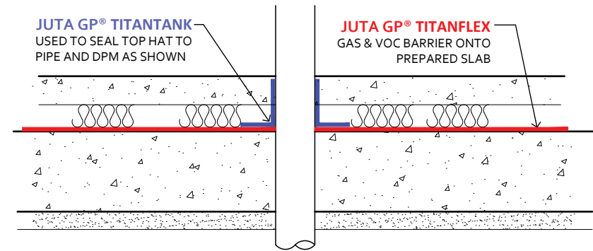
PIPE PENETRATION WITH SELF ADHESIVE GAS MEMBRANE
